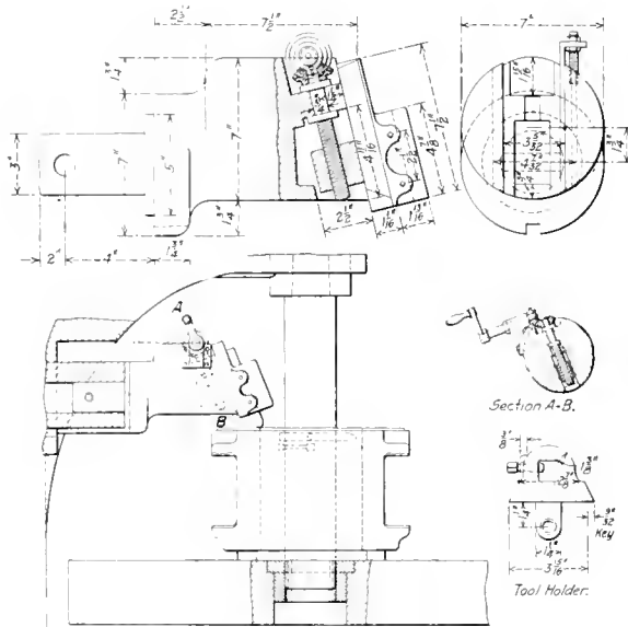
Car Wheel Borer, Arranged for Machining Driving Boxes
